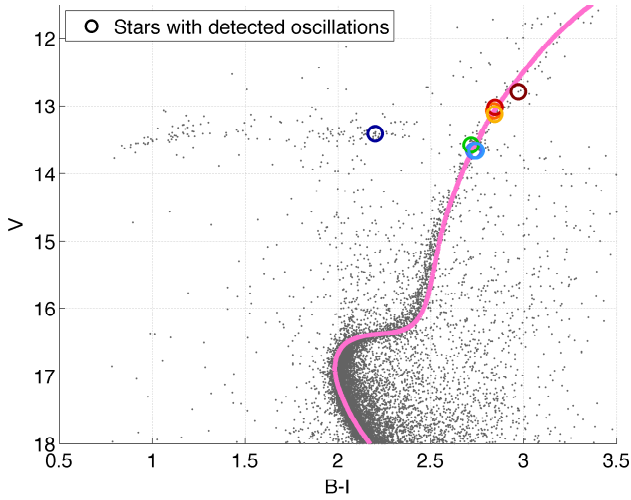
Figure 1. Colour magnitude diagram of M4 stars based on the dataset described in D’Antona et al. (2009). Magnitudes and colour were corrected for differential reddening following Milone et al. (2012). The solid line represents a isochrone (from BaSTI, see Sec. 3.1.1 for details) fit to the CMD. The large coloured open circles mark the stars with detected solar-like oscillations (the corresponding oscillation spectra are plotted in Fig. 2).
