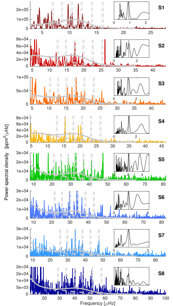
Figure 2. Solar-like oscillation spectra of eight K giants observed by K2. The bottom star is in the RHB. Stars (from top to bottom) are ordered by increasing \nu_{\max} . Vertical lines show the position of radial (dashed lines) and quadrupole (dash-dotted lines) oscillation frequencies as expected by the pattern of oscillation modes in red-giant stars described in Mosser et al. (2011). The expected granulation power and the combined granulation and oscillation power is represented by dashed and solid thick lines. The insets show the power spectrum of the power spectrum (PSPS) of each star, computed from the region around \nu_{\max} . In each PSPS the prominent peak at \Delta\nu/2 (vertical gray line) is the detected signature of the near-regular spacing of oscillation peaks in the frequency spectrum.
