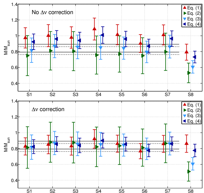
Figure 3. Mass of M4 giants as inferred from Eq. 1 to 4 with (lower panel) and without (upper panel) applying a model-predicted correction to the \Delta\nu scaling relation. The last star to the right (S8) is a RHB star. The solid and dashed lines denote the 1\text{-}\sigma mass interval as determined from isochrone fitting and assuming two values for the initial He mass fraction (see Section 3.1.1 for details).
